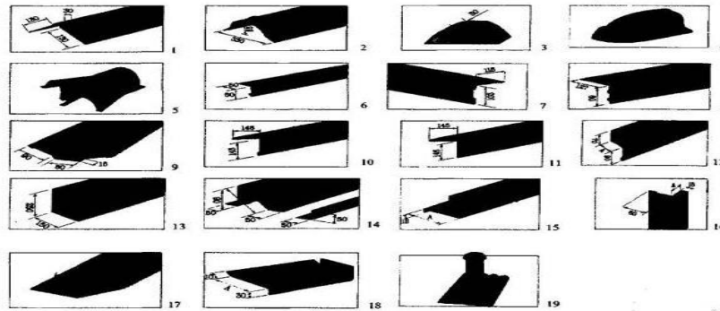
1 - rod; 2 - crest strip designed for the Monterrey profile; 3 - termination for the crest strip; 4 - termination for the hip roof crest strip; 5 - "U" shaped strip for the termination of the hip roof; 6 - termination strip measuring 50×50 mm; 7 - termination strip sized at 103×115 mm; 8 - eave strip; 9 - strip for internal seams and joints; 10 - strip for external corners; 11 - strip for internal corners; 12 - versatile strip featuring both internal and external corners; 13 - strip for seams and joints; 14 - snow retention device; 15 - upper rod; 16 - lateral rod; 17 - strip for grooves; 18 - sheet for covering external recesses; 19 - drainage pipe exit.
